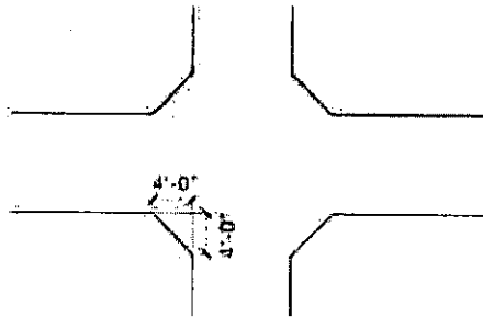
Exhibit 3 Chamfered Intersection
