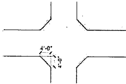
Exhibit 4-8.3 Chamfered Intersection
